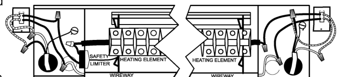
BKT2A/BKT2BW wiring diagram
