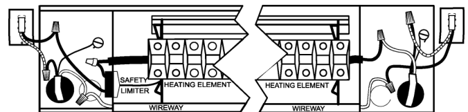
BKT1A/BKT1BW wiring diagram
