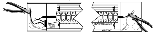
Factory wire splice cutting diagram
